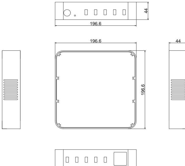
Machine Dimensions ( Unit: mm)
