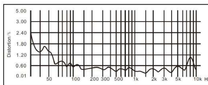
Distortion Characteristics (THD < 3% 1W, 1m, 100Hz-10kHz)
