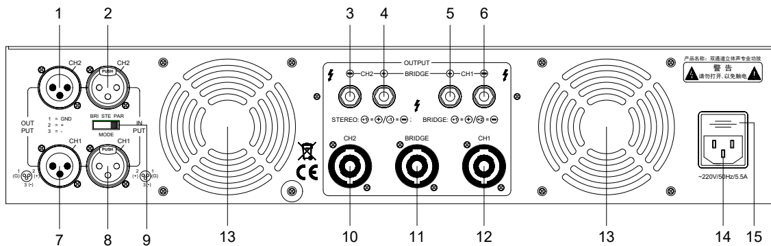
DX2000/DX2500 Rear Panel
